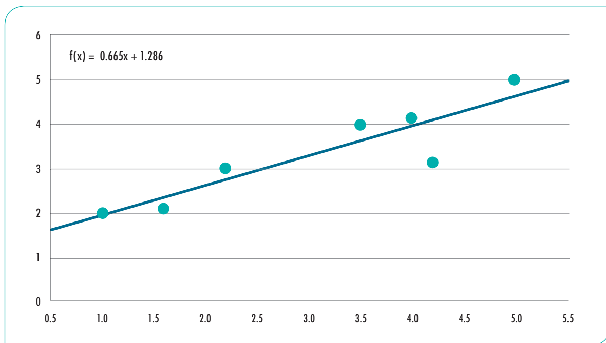
Figure 4.10: Linear regression.
