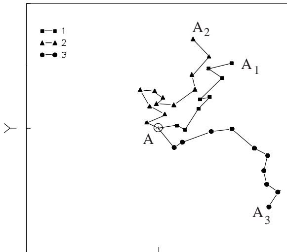
Figure 3. Final position of three particles after ten time steps.
