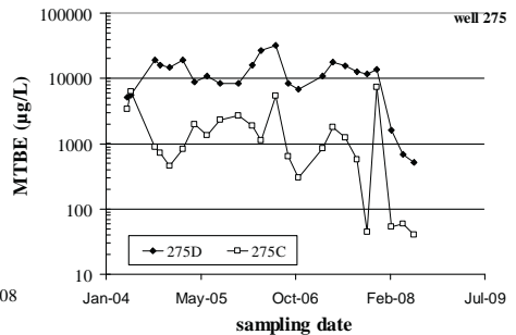
Figure 3. Concentrations of MTBE in monitoring wells “275”. C and D indicate screen depths (D is the deeper screen, ref. to Figure 1)
