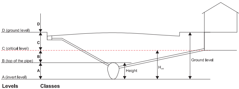
Figure 1. Overview of levels, classes and altitudes for pipe classification
