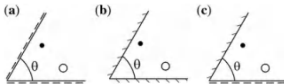
Fig. A3.5 Schematic planar view of a wedge-shaped aquifer. a Two constant-head boundaries; b two impermeable boundaries; c combined boundary conditions
