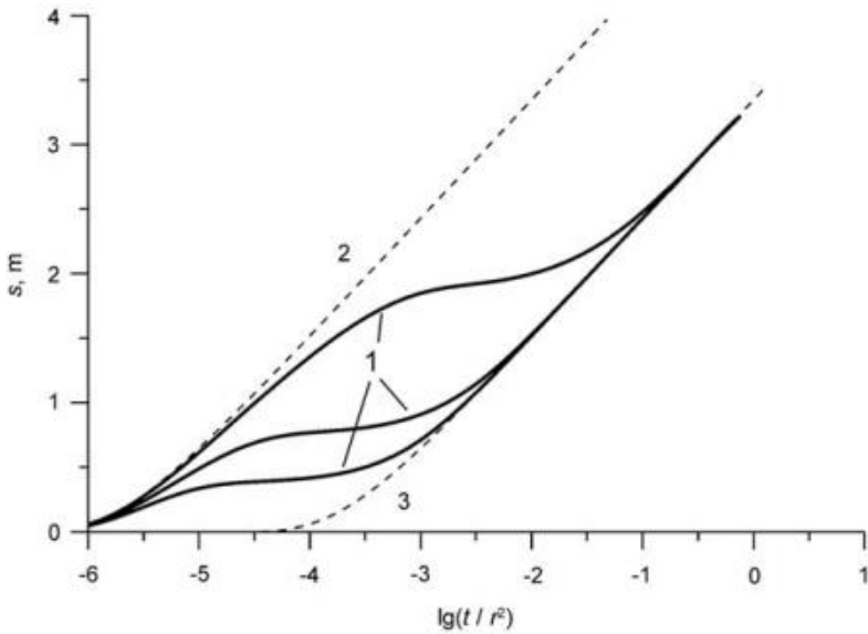
Fig. 12.18 Time-distance-drawdown plot for an unconfined aquifer (curve 1). The plot is drawn for three observation wells based on the Boulton solution (Eq. 2.10). The thin dashed lines are the Theis solution (Eq. 1.1) assuming an elastic storage coefficient (curve 2) and a specific yield of an unconfined aquifer (curve 3)
