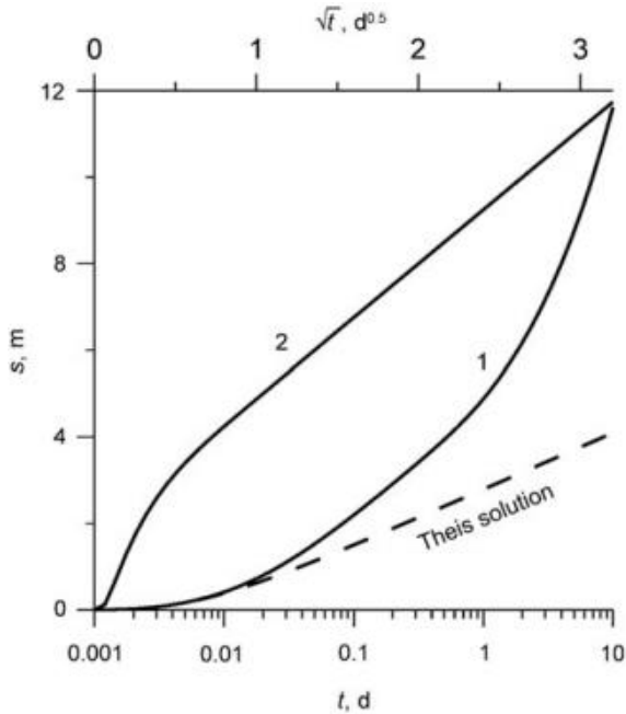
Fig. 12.14 The drawdown in a strip aquifer with impermeable boundaries: (curve 1) in coordinates s\text{---}\lg t , (curve 2) in coordinates s\text{---}\sqrt{t}
