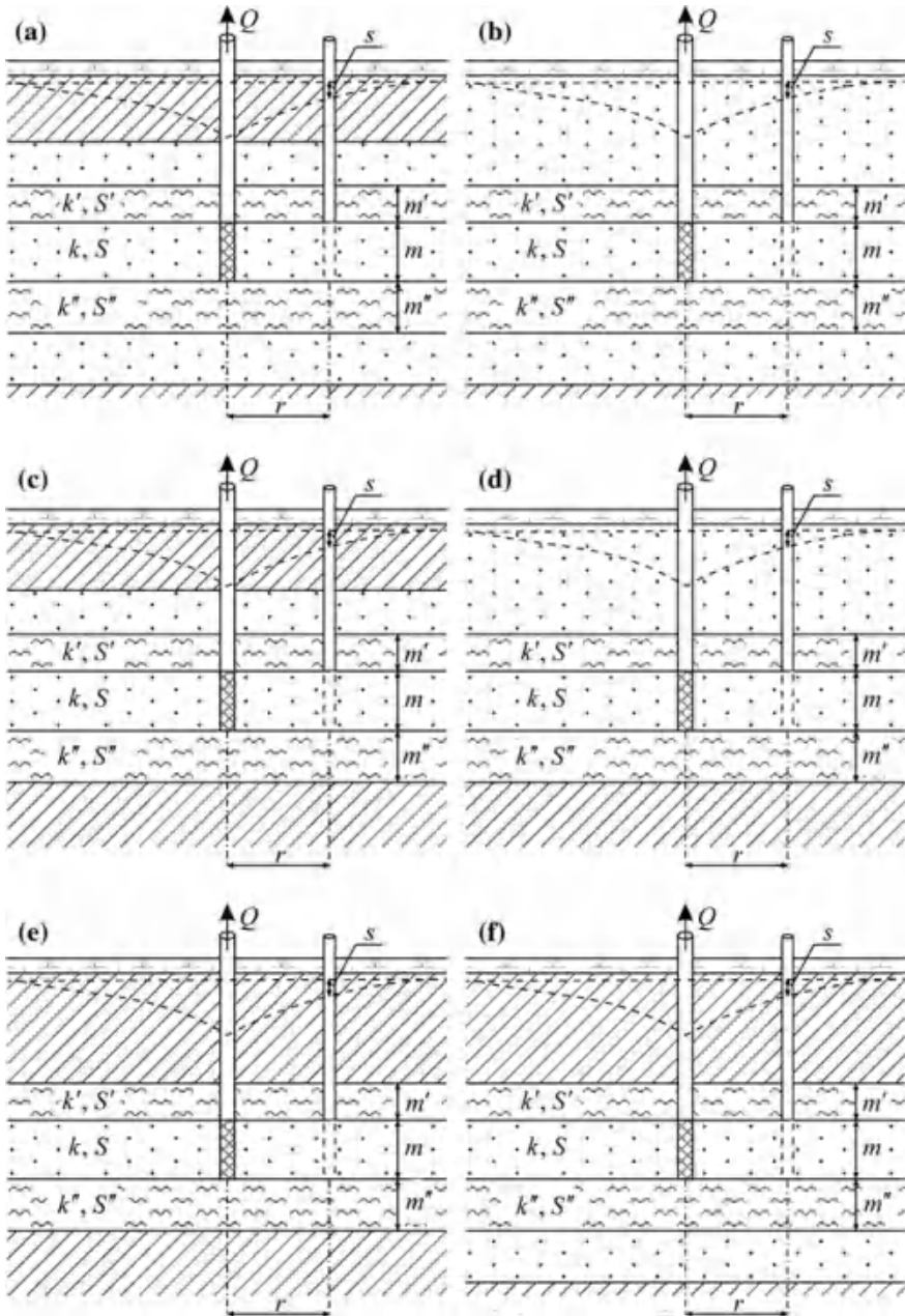
Fig. 3.15 Three-layer systems: a, b the top and bottom are constant-head aquifers—a a confined aquifer in the top, b an unconfined aquifer in the top; c, d the top is a constant-head aquifer (c confined, d unconfined), the bottom is an aquiclude; e the top and bottom are aquicludes; f an aquiclude in the top, a constant head aquifer in the bottom
