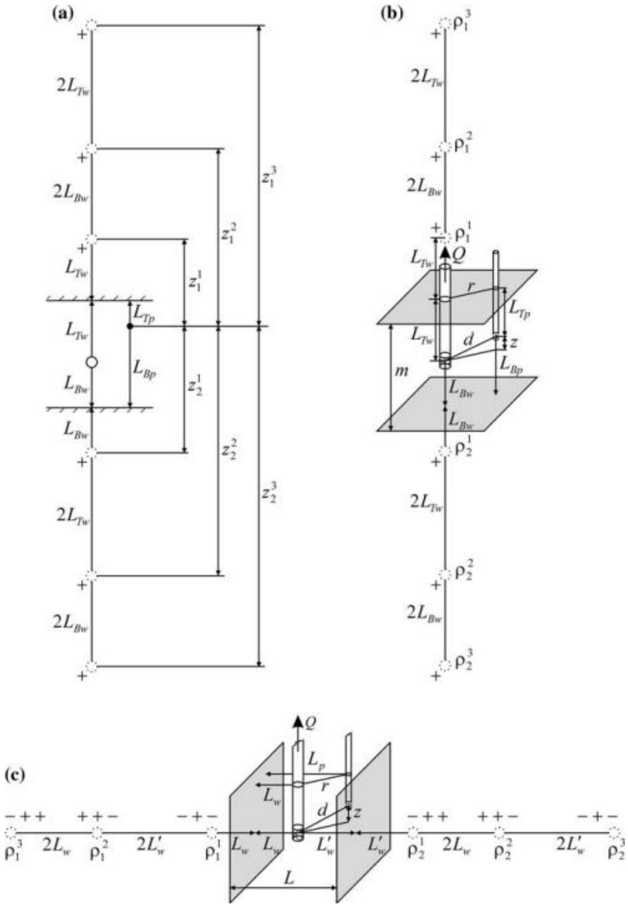
Fig. A3.12 Schemes for evaluating the distances to image wells for point and linear sources. a Cross-section for a linear source, the circle, and the dot in the section are the centers of the pumping and observation wells, respectively; b, c three-dimensional schemes for a point source in an aquifer limited in b thickness and c the plane. For explanations of discharge signs, see in Fig. A3.4
