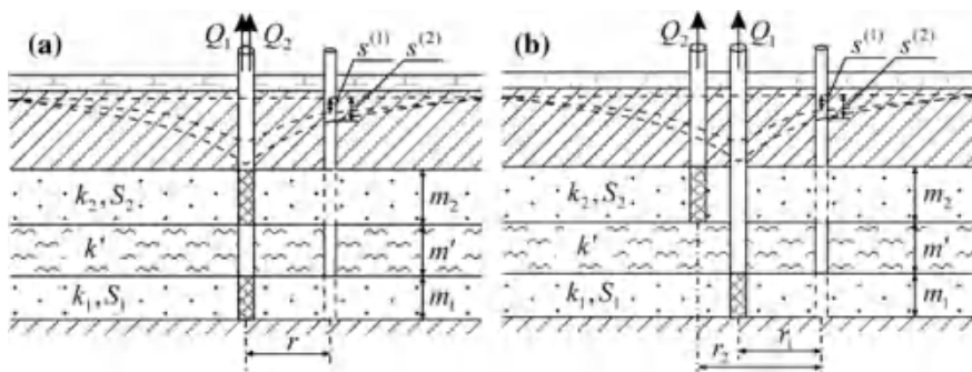
Fig. 10.3 Leaky aquifers with pumping from two aquifers through a single pumping well with two screens and b two wells
