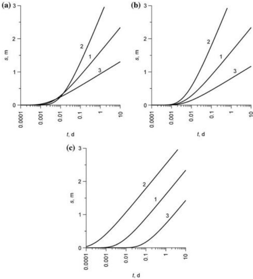
Fig. 12.10 The effect of hydraulic parameters on the drawdown in a confined aquifer: a transmissivity ( T_2 \setminus T_1 \setminus T_3 ) at constant storage coefficient; b transmissivity ( T_2 \setminus T_1 \setminus T_3 ) at constant hydraulic diffusivity; c storage coefficient ( S_2 \setminus S_1 \setminus S_3 ) [or hydraulic diffusivity ( a_3 \setminus a_1 \setminus a_2 )] at constant transmissivity. The numbers at the curves (1, 2, 3) correspond to the subscripts at hydraulic characteristics
