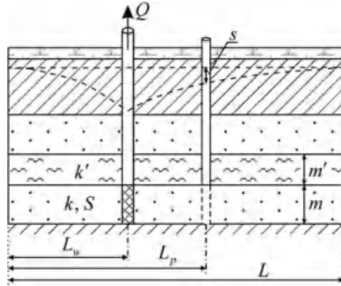
Fig. 3.5 A leaky aquifer, bounded by two parallel boundaries (strip aquifer). L is the width of the strip aquifer
