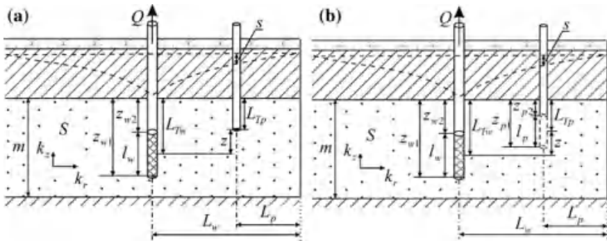
Fig. 1.23 A linear source in a confined semi-infinite in the horizontal plane aquifer. Schematic cross-sections: a with a piezometer, b with an observation well
