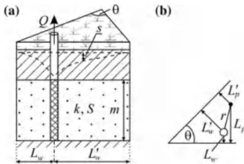
Fig. 1.6 Wedge-shaped confined aquifer: a cross-section and b planar view. L'_w ; L'_p are the distances from the pumping and observation wells to the second boundary, respectively; h is the angle between two intersecting boundaries
