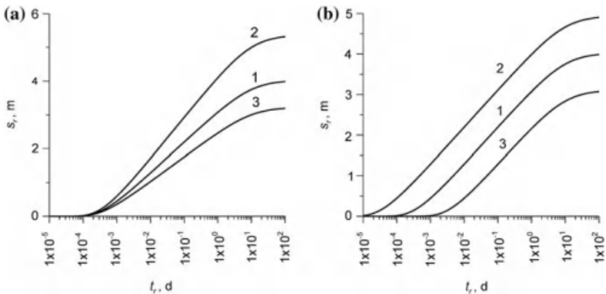
Fig. 12.33 The effect of hydraulic characteristics on recovery (the water level is measured from the end of pumping) (Eq. 11.12): a transmissivity ( T_2 \setminus T_1 \setminus T_3 ); b storage coefficient (or hydraulic diffusivity) ( S_2 \setminus S_1 \setminus S_3 or a_3 \setminus a_1 \setminus a_2 ). The numbers at the curves (1, 2, 3) correspond to the subscripts at hydraulic characteristics. s_r is level recovery measured from the dynamic level at the moment when pumping was stopped
