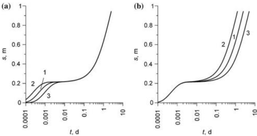
Fig. 12.20 Time-drawdown plot for an unconfined aquifer. The effect of hydraulic characteristics: a specific storage ( S_2 \setminus S_1 \setminus S_3 ); b specific yield ( S_{y2} \setminus S_{y1} \setminus S_{y3} ). The numbers on the curves (1, 2, 3) correspond to subscripts at hydraulic characteristics
