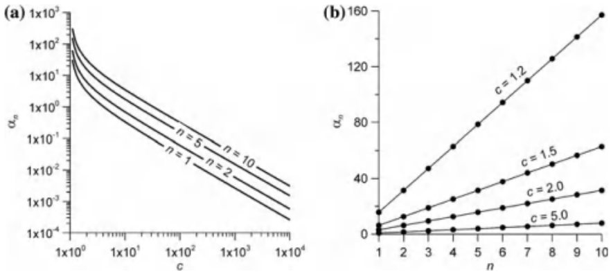
Fig. A7.28 Roots of equation J_0(a_n) Y_0(ca_n) - Y_0(a_n) J_0(ca_n) = 0 . a Dependence of the logarithm of the root (1st, 2nd, 5th, and 10th) on the logarithm of c and b dependences of the root on its number at different c (1.2, 1.5, 2.0, and 5.0). c is a constant; n is the root's number
