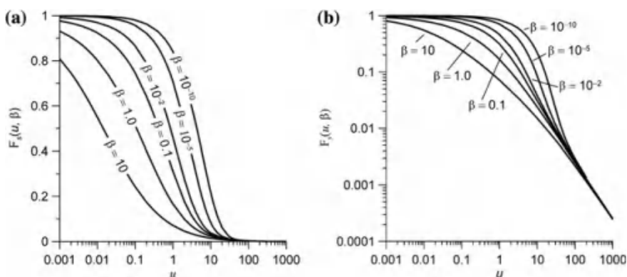
Fig. A7.12 Plots of function F_s(u, b) at different values of its second argument: a F_s(u, b) - \lg(u) , b \lg[F_s(u, b)] - \lg(u)
