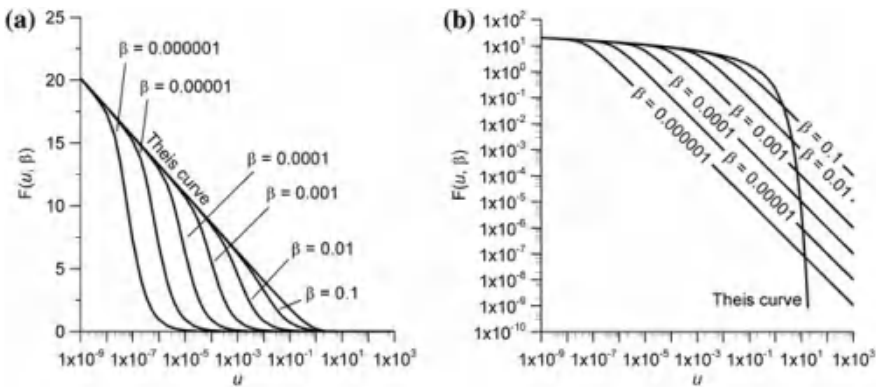
Fig. A7.10 Plots of a the function and b the logarithm of the function F(u, b) versus the logarithm of the first argument at different values of its second argument
