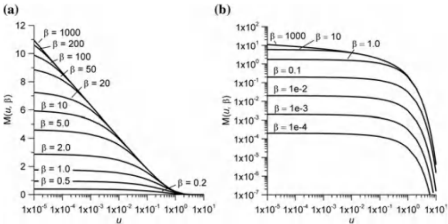
Fig. A7.3 Plots of function M(u, b) at different values of its second argument: a M(u, b) - \lg(u) , b \lg[M(u, b)] - \lg(u)
