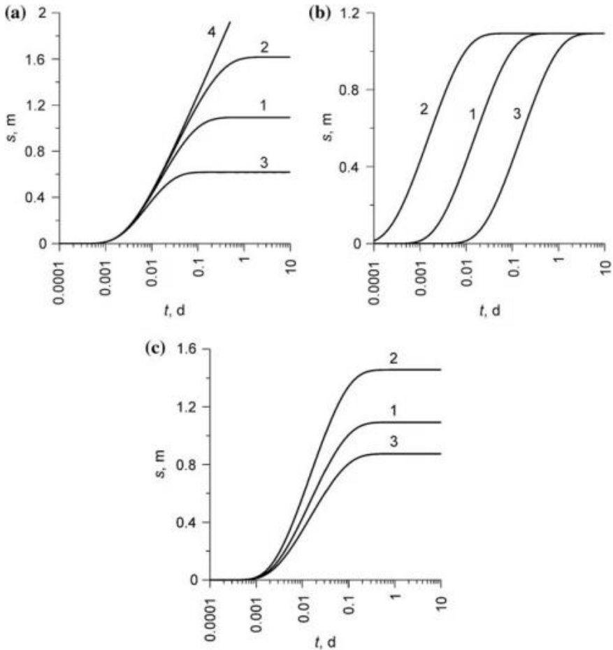
Fig. 12.21 Time–drawdown plots for a leaky aquifer: Hantush–Jacob solution (Eq. 3.1). The effect of hydraulic characteristics: a leakage factor ( B_3 \setminus B_1 \setminus B_2 ); b hydraulic diffusivity ( a_3 \setminus a_1 \setminus a_2 ); c transmissivity ( T_2 \setminus T_1 \setminus T_3 ). As B_4 \rightarrow \infty , the Hantush–Jacob solution tends to the Theis solution (Eq. 1.1). The numbers on the curves (1, 2, 3, 4) correspond to subscripts at hydraulic characteristics
