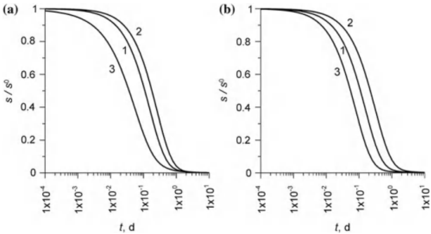
Fig. 12.31 Normalized water-level recovery versus time for slug tests. The effect of hydraulic characteristics: a storage coefficient ( S_2 \setminus S_1 \setminus S_3 ); b transmissivity ( T_2 \setminus T_1 \setminus T_3 ). The numbers at the curves (1, 2, 3) correspond to the subscripts at hydraulic characteristics
