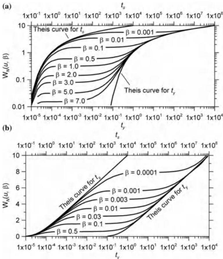
Fig. A7.6 Plots of function W_N(u, b) at different values of its second argument: a \lg[W_N(u, b)] - \lg(u) , b W_N(u, b) - \lg(u) . The top scale is for u = t_s , the bottom scale, for u = t_y
