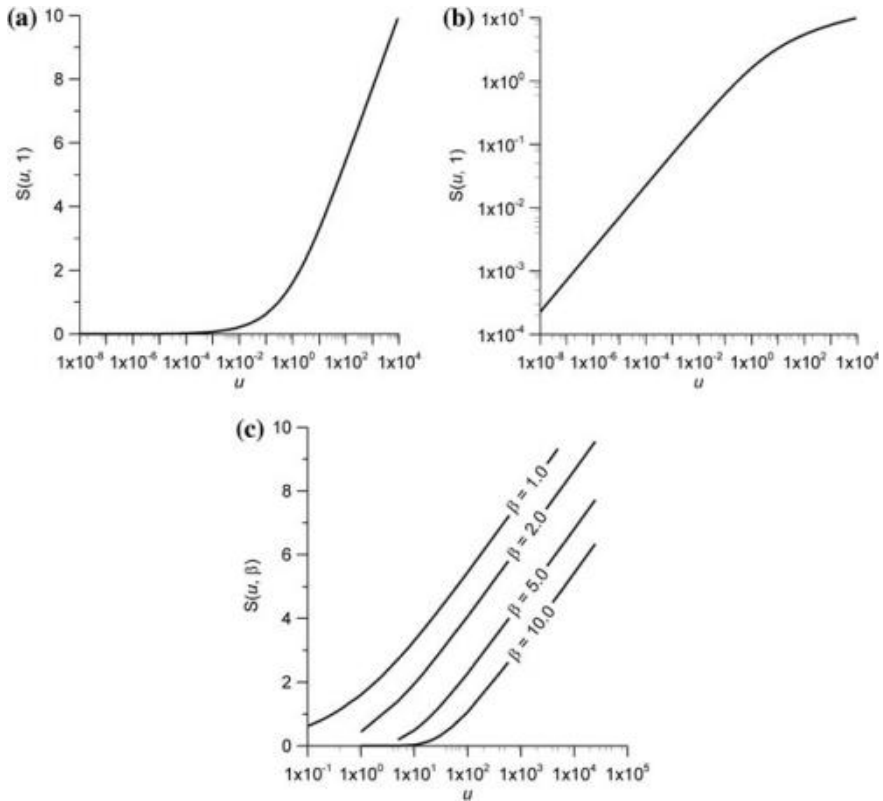
Fig. A7.11 Plots of function S(u, b) at b = 1 : a S(u, b) - \lg(u) ; b \lg[S(u, b)] - \lg(u) . c Plot of function S(u, b) - \lg(u) at different values of its second argument
