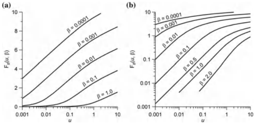
Fig. A7.5 Plots of function F_B(u, b) at different values of its second argument: a F_B(u, b) - \lg(u) , b \lg[F_B(u, b)] - \lg(u)
