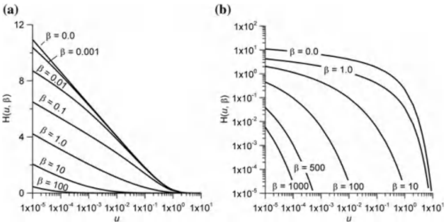
Fig. A7.4 Plots of function H(u,b) at different values of its second argument: a H(u, b) - \lg(u) , b \lg[H(u, b)] - \lg(u)
