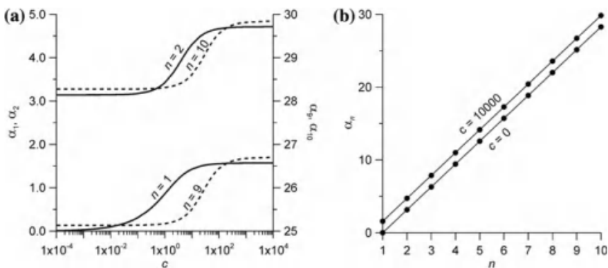
Fig. A7.24 Roots of equation a_n \tan(a_n) = c . Dependence of the root (1st, 2nd, 9th, and 10th) on a c and b its number n at different values of c (0 and 10000). c is a constant; n is the root's number
