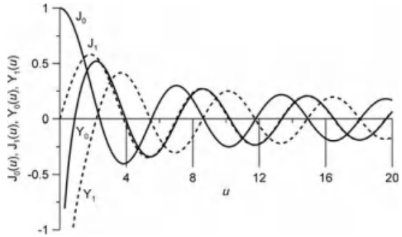
Fig. A7.18 Plots of Bessel functions: J_0(u) , J_1(u) , Y_0(u) , Y_1(u)
