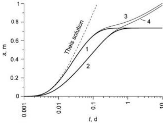
Fig. 12.22 Time-drawdown plots for leaky aquifers: (curve 1) the water level in the adjacent aquifer is constant—the Hantush–Jacob solution (Eq. 3.1); (curve 2) the water level in the adjacent aquifer is constant, aquitard storage is taken into account (Eq. 3.67); (curve 3) the water level in the adjacent aquifer is variable (Eq. 3.40); (curve 4) the water level in the adjacent aquifer is variable, aquitard storage is taken into account (Eq. 3.73)
