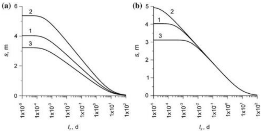
Fig. 12.32 The effect of hydraulic characteristics on recovery (the water level is measured from the start of pumping) (Eq. 11.9): a transmissivity ( T_2 \setminus T_1 \setminus T_3 ); b storage coefficient (or hydraulic diffusivity) ( S_2 \setminus S_1 \setminus S_3 or a_3 \setminus a_1 \setminus a_2 ). The numbers at the curves (1, 2, 3) correspond to the subscripts at hydraulic characteristics. t_r is time measured from the start of recovery
