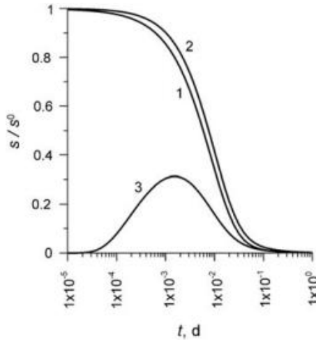
Fig. 12.30 Normalized water-level recovery versus time for a slug test: Cooper solution for the tested well (Eq. 9.1)—an instantaneous change in the initial water level (curve 1); Picking solution (Eq. 9.5), taking into account a delay in the change in initial level (curve 2); Cooper solution of an observation well (curve 3) (Eq. 9.3)
