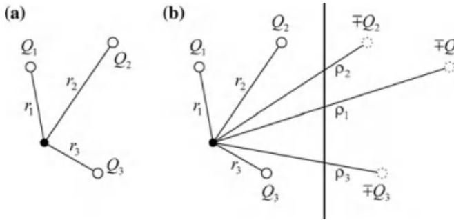
Fig. 10.1 Example of layout of three pumping wells for a multi-well constant-discharge test in an aquifer with a infinite and b semi-infinite lateral extent. The signs of the discharge rates of the image wells are minus for a constant-head boundary and plus for an impermeable boundary
