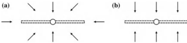
Fig. 6.3 Schemes (planar view) of a pseudo-radial and b linear flow toward a vertical fracture
