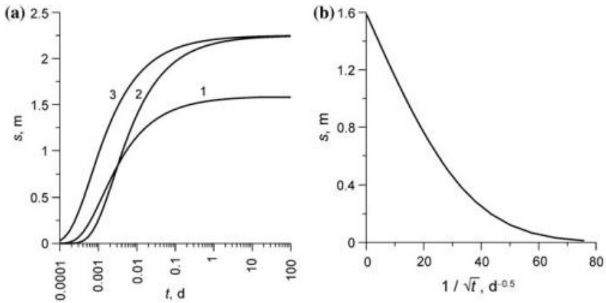
Fig. 12.15 Time-drawdown plots for a point source in a confined aquifer infinite in the horizontal plane and thickness (Eq. 1.79): a in coordinates s\text{--}lgt ; b in coordinates s\text{--}1=\sqrt{t} . (curve 1) isotropic aquifer, (curve 2) anisotropic aquifer ( k_r < k_z ), and (curve 3) anisotropic aquifer ( k_r > k_z )
