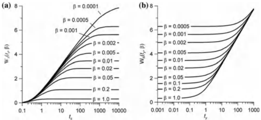
Fig. A7.7 Plots of function W_N(u, b) at different values of its second argument: a W_N(t_s, b) - \lg(t_s) , b W_N(t_y, b) - \lg(t_y)
