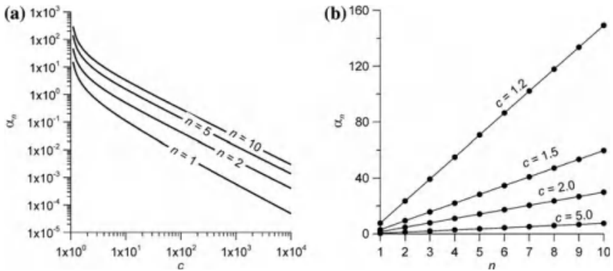
Fig. A7.29 Roots of equation J_0(a_n) Y_1(ca_n) - Y_0(a_n) J_1(ca_n) = 0 . a Dependence of the logarithm of the root (1st, 2nd, 5th, and 10th) on the logarithm of c and b dependences of the root on its number at different c (1.2, 1.5, 2.0, and 5.0). c is a constant; n is the root's number
