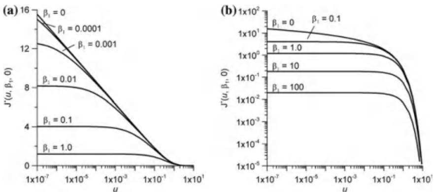
Fig. A7.8 Plots of function J^*(u, b_1, b_2) for b_2 = 0 : a J^*(u, b_1, 0) - \lg(u) , b \lg[J^*(u, b_1, 0)] - \lg(u) . b_2 = 0 implies that the pumping and observation wells are located on a perpendicular to the river
