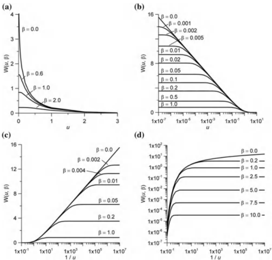
Fig. A7.2 Plots of function W(u, b) at different values of its second argument: a W(u, b) - u , b W(u, b) - \lg(u) , c W(u, b) - \lg(1/u) , d \lg[W(u, b)] - \lg(1/u)
