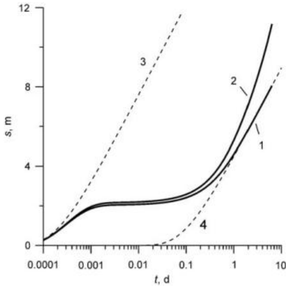
Fig. 12.19 Time-drawdown plot for an unconfined aquifer. Solution without correction (curve 1); corrected drawdown (curve 2). The thin dashed lines are Theis solution (Eq. 1.1) assuming an elastic storage coefficient (curve 3) and a specific yield of unconfined aquifer (curve 4)
